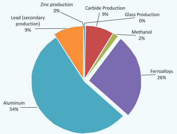
CO 2 Emissions from Industrial activities other than Cement in Himachal Pradesh
