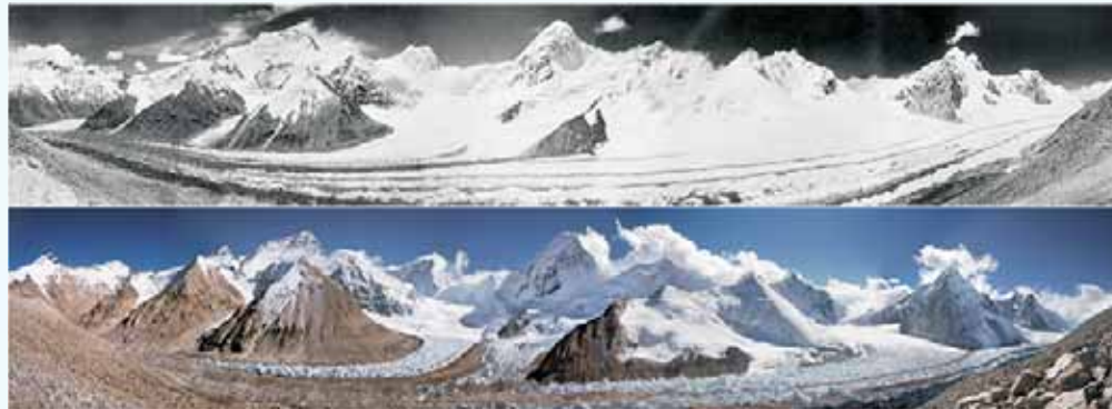
Panoramic View of West Rongbuk Glacier during an analysis of Everest between 1921 and 2009 taken in 1921 (top) by Major E.O. Wheeler and in 2009 (bottom) by David Breashears.
