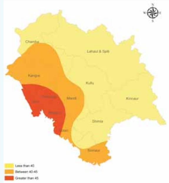
Fig. 13(ii): Highest Temperature Ever Recorded (°C)
