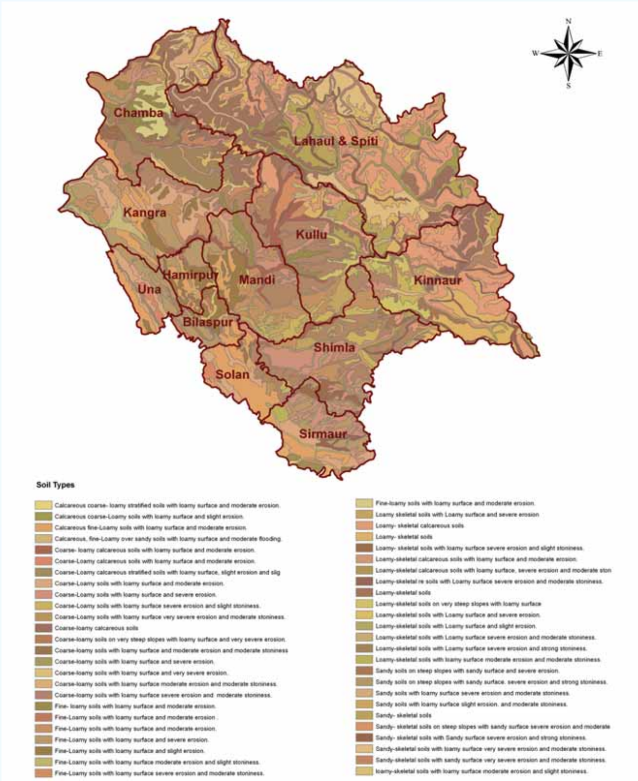
Fig. 7: Soil Classification Map of Himachal Pradesh
