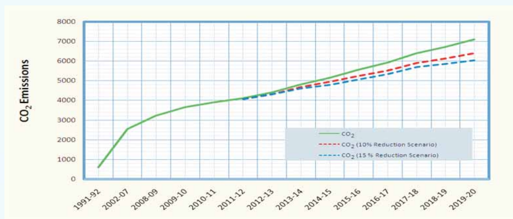
Fig. 43: CO 2 Emissions as per Energy Demand Projections
