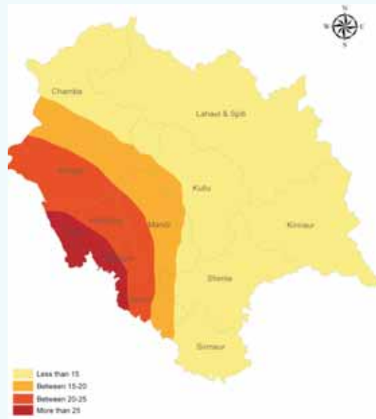
Fig. 23 Annual Normal Temperature (°C)
