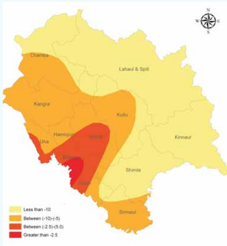
Fig. 13(iii): Lowest Minimum Temperature Ever Recorded (°C)
