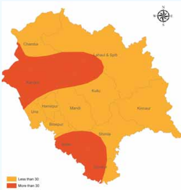
Fig. 28(i) Mean Max. Temperature (°C) - August
