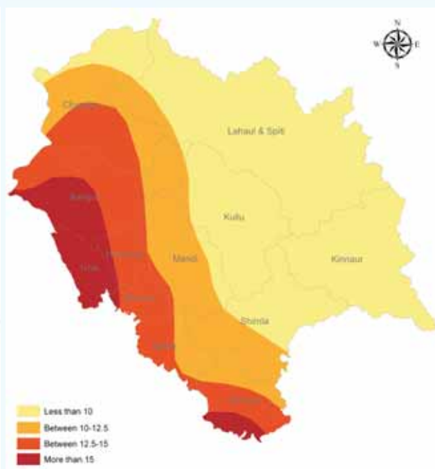
Fig. 27 Mean Minimum Temperature (°C) - October
