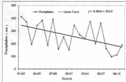
Fig. 11 (i): Total Seasonal Precipitation over Shimla
