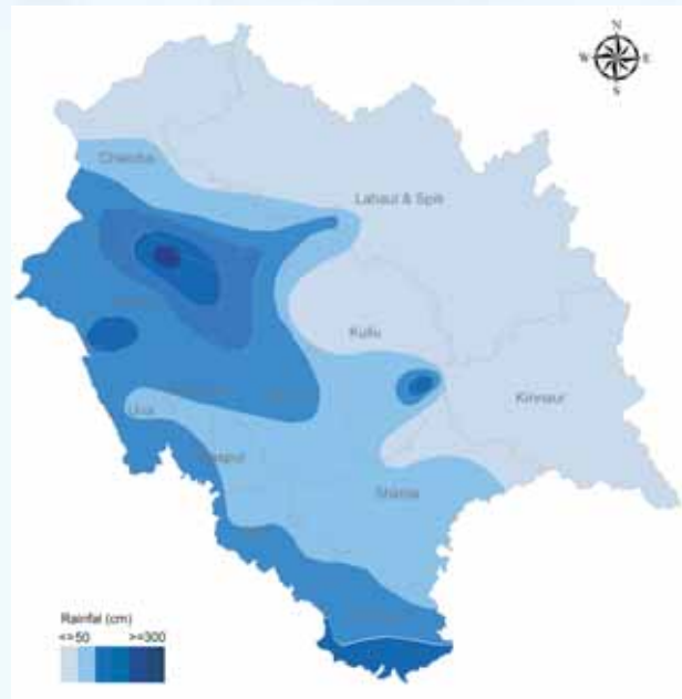
Fig. 15(iv): Monsoon Season- June to September
